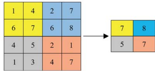
Fig. 3. Pooling operation
